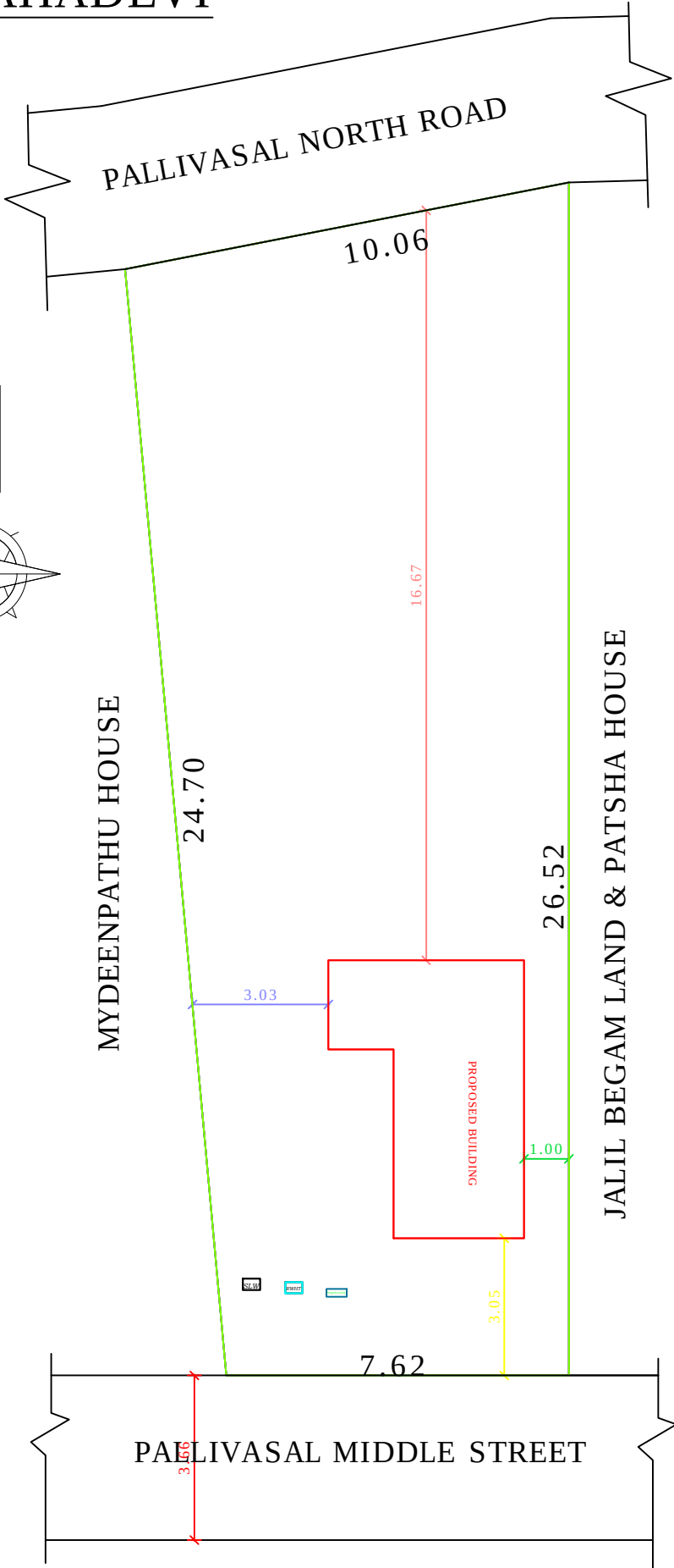
SITE PLAN
