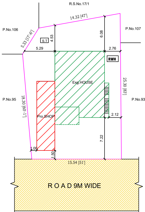
TOPO PLAN ( Not to Scale )
