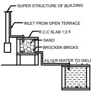
DETAILS OF FILTER BED & WELL
