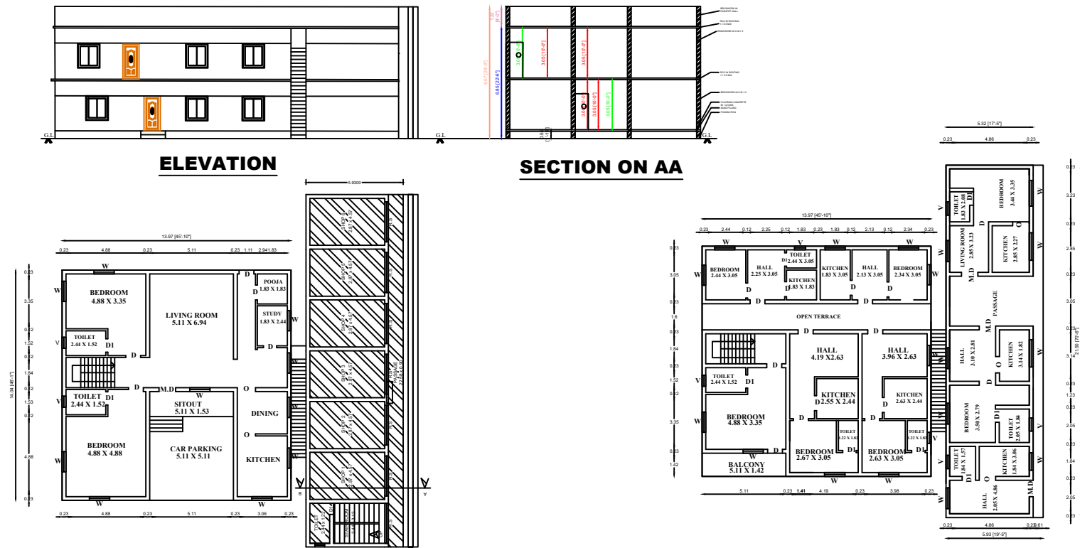
PRO RESIDENTIAL FIRST FLOOR PLAN ( ESAKKIAMMAN KOVIL ) SOMASUNDARAM LAND
