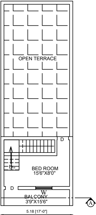
RST FLOOR PLAN
