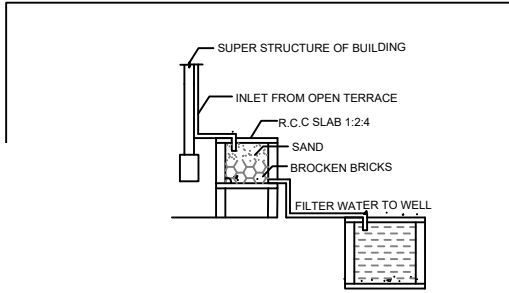
DETAILS OF FILTER BED & WELL NTS
