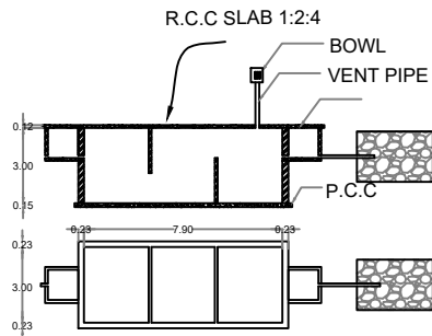
SEPTIC TANK AND TRENCH NTS
