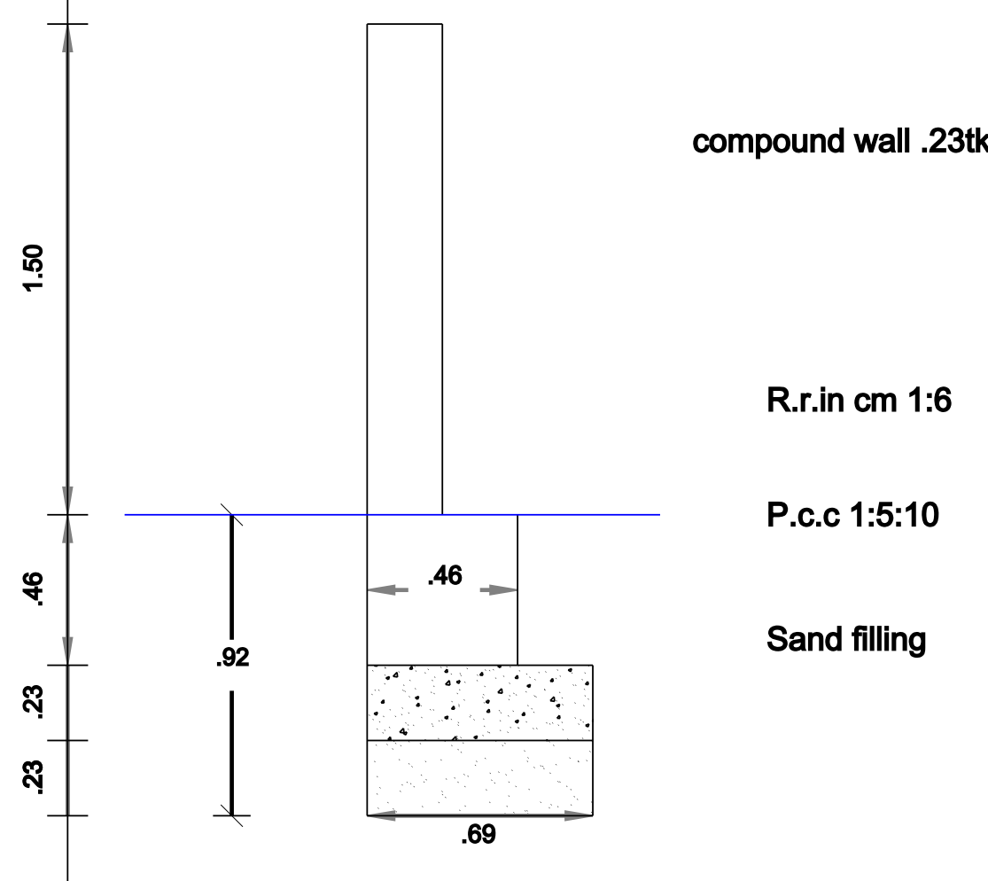
Compound Wall Detail
