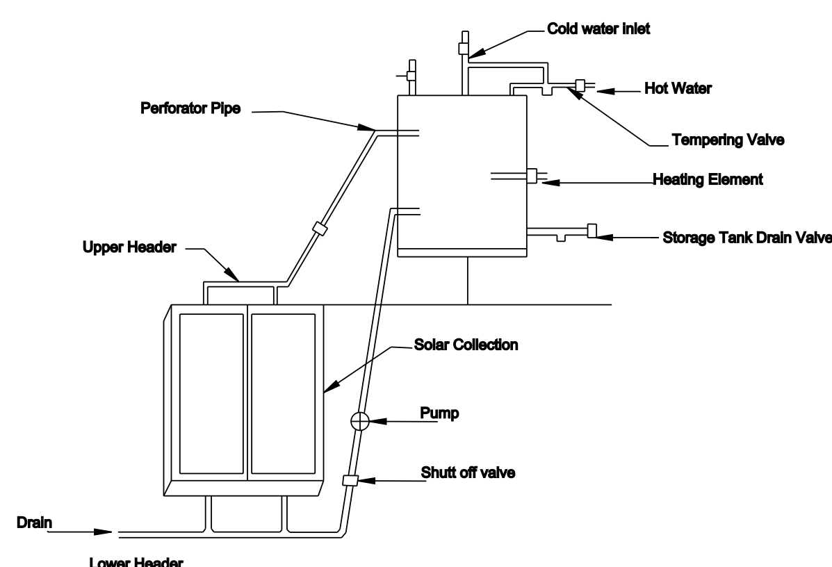
Details Of Solar Water Heater (NTS)
