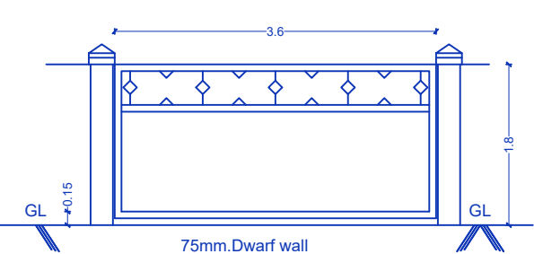
COMPOUND WALL ENTRANCE GATE
