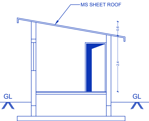
SECTION
