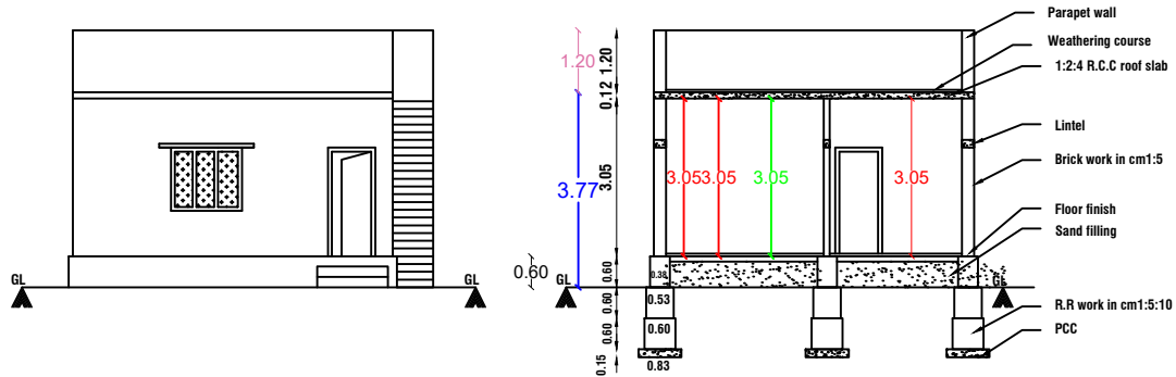
FRONT ELEVATION
