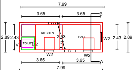
GROND FLOOR PLAN
