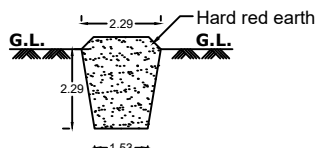
TRIAL PIT (Scale 1:100)
