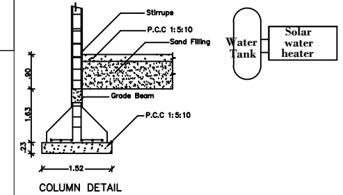
COLUMN DETAIL
