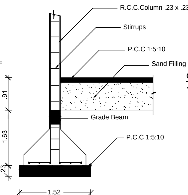
COLUMN DETAIL
