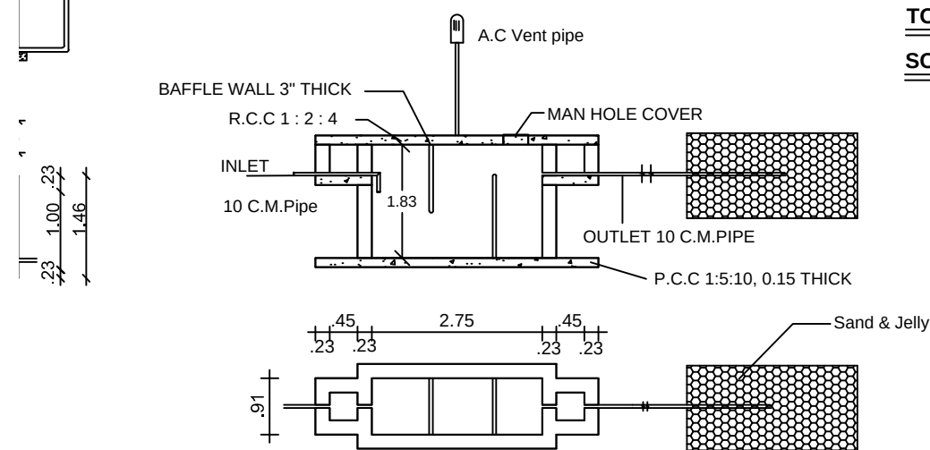
SEPTIC TANK AND TRENCH
