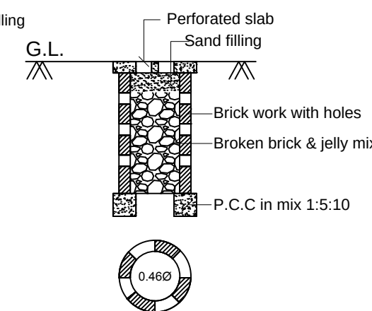
PERCOLATION PIT FOR 30 Sq. m.
