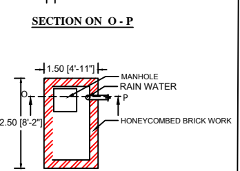
PLAN RAIN WATER HARVESTING
