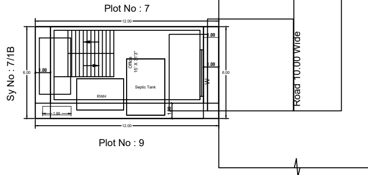
SITE PLAN
