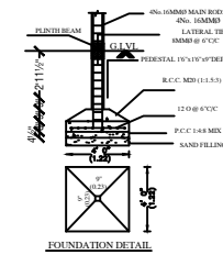
FOUNDATION DETAIL
