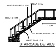
STAIRCASE DETAILS
