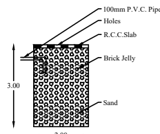
SECTION OF RAIN WATER COLLECTING TANK
