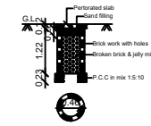
PERCOLATION PIT FOR 30 Sq. m. (Scale:- 1:50)
