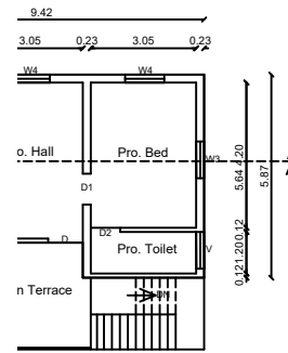
T FLOOR PLAN
