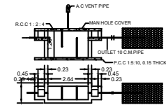
SEPTIC TANK DETAILS
