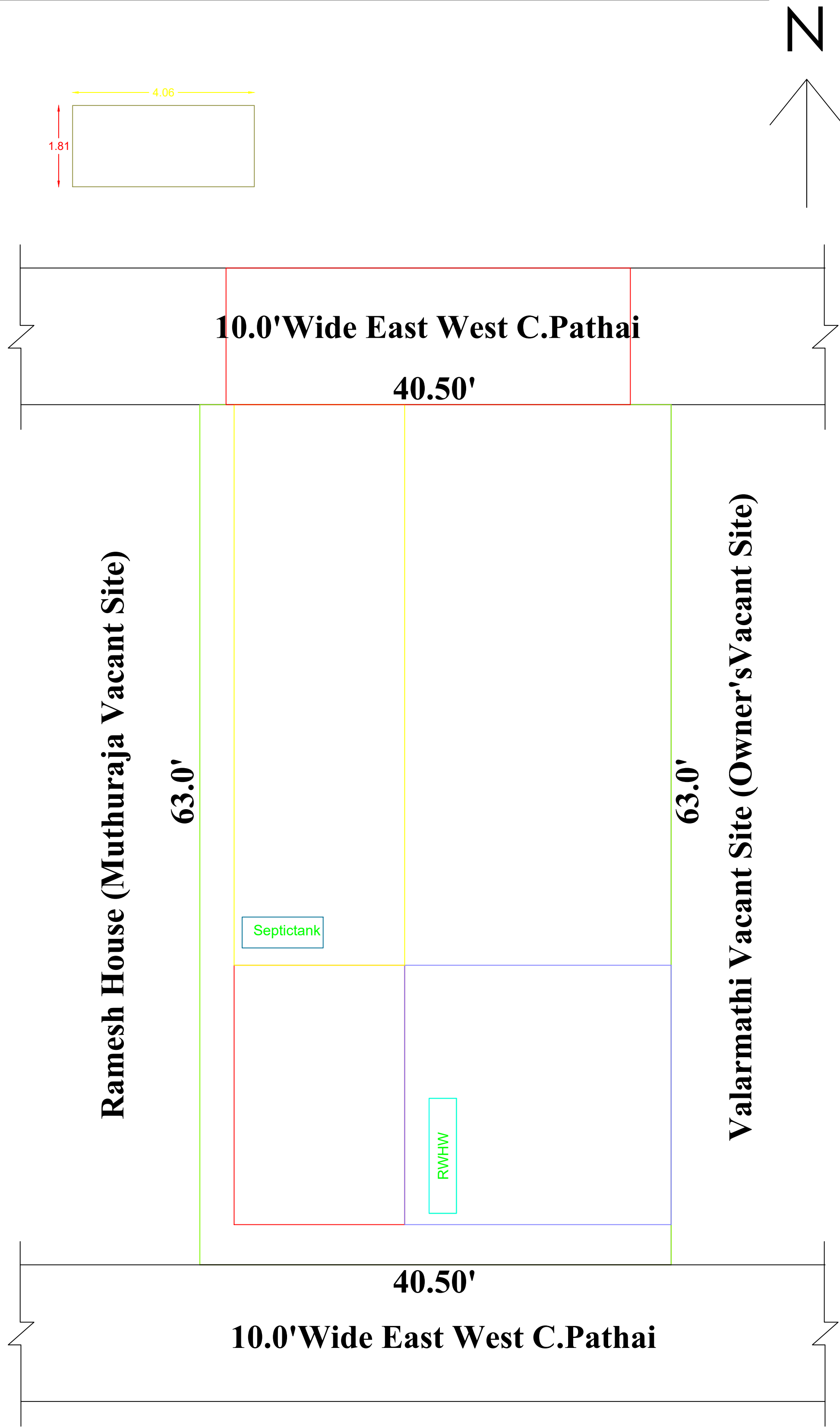
SITE PLAN
