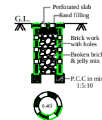
PERCOLATION PIT (NOT FOR SCALE)
