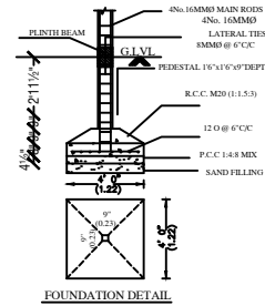
FOUNDATION DETAIL
