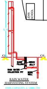
RAIN WATER HARVESTING SYSTEM
