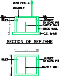
PLAN SEPTIC TANK
