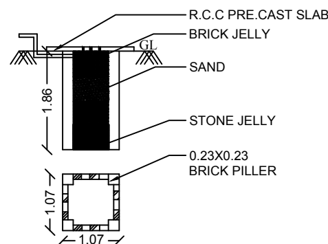
PLAN AND SECTION OF RAINWATER COLLECTION WELL
