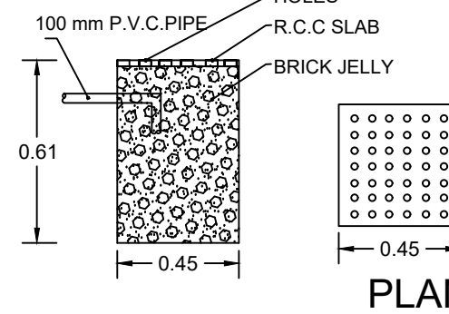
SECTION OF RAIN WATER PIT
