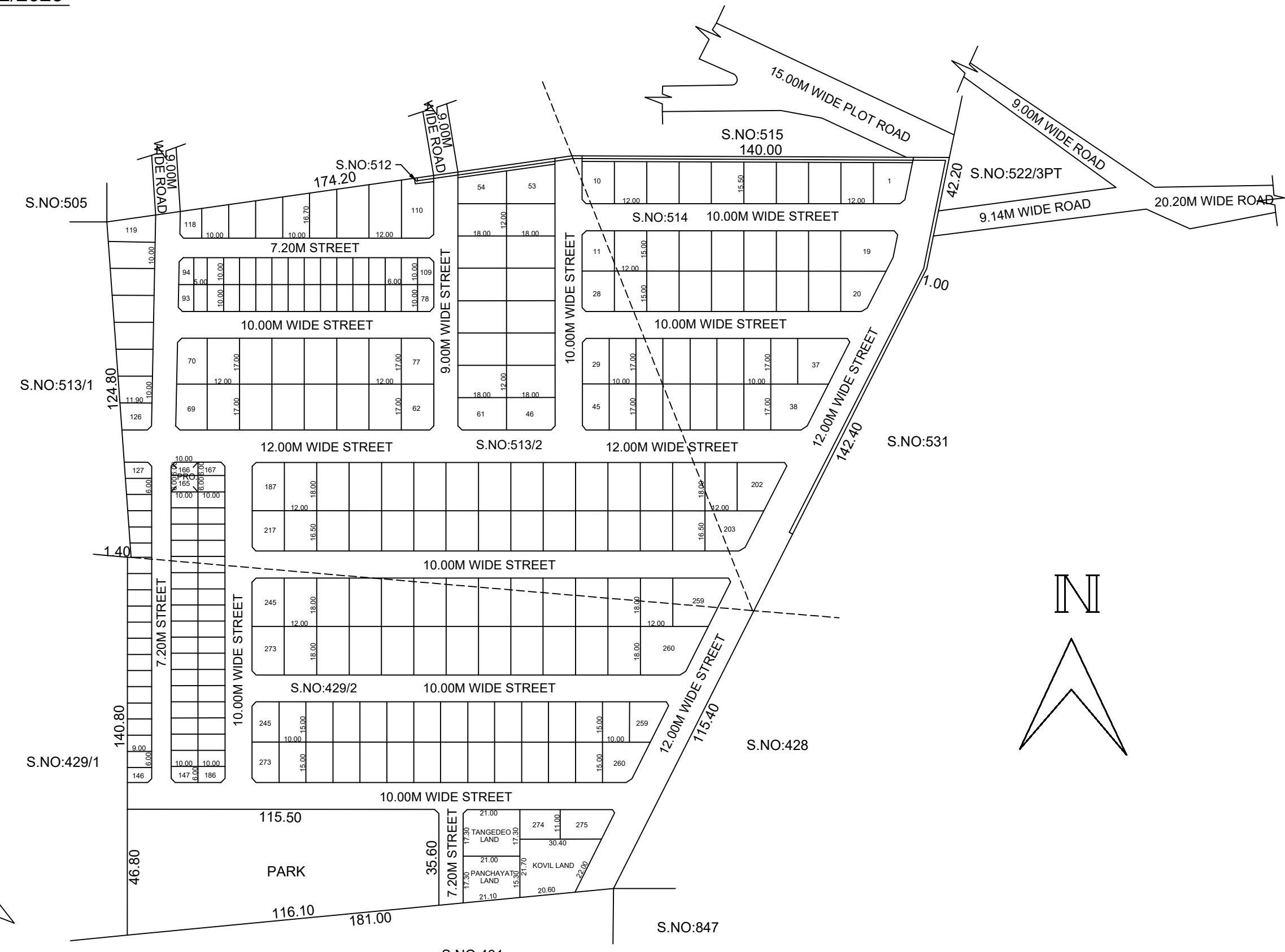
TOPO PLAN (NOT TO SCALE)
