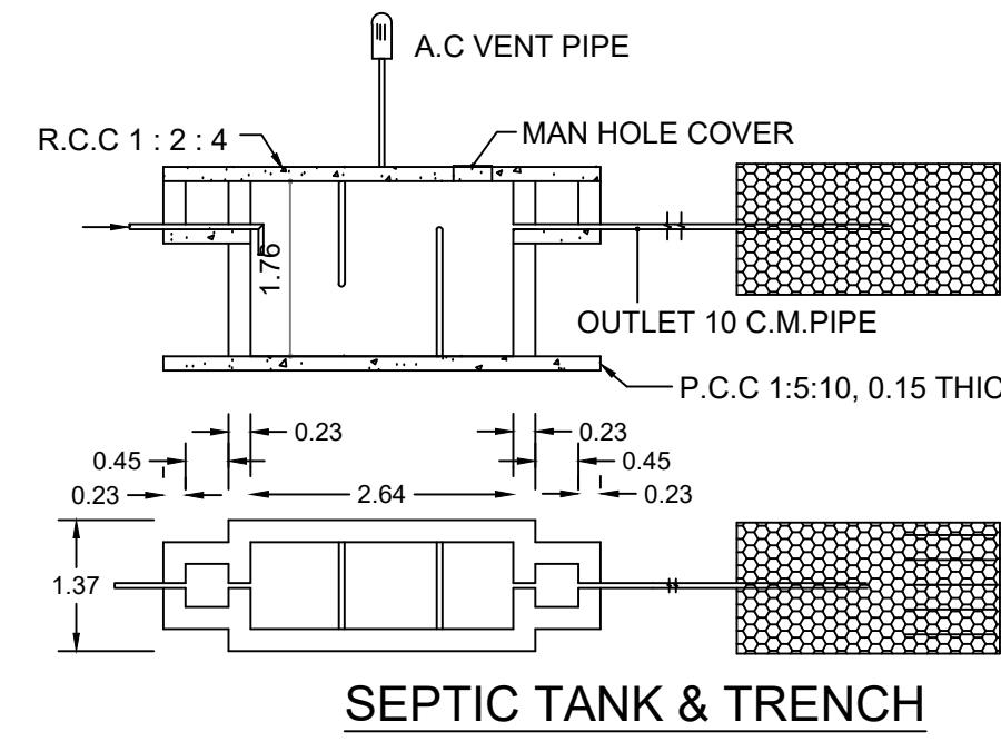
SEPTIC TANK & TRENCH
