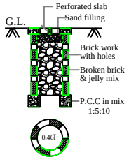
PERCOLATION PIT (NOT FOR SCALE)
