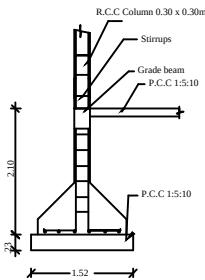
Column Detail
