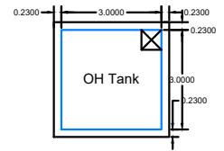
WATER TANK CAPACITY L=13500LTRS
