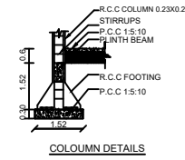
COLOUMN DETAILS
