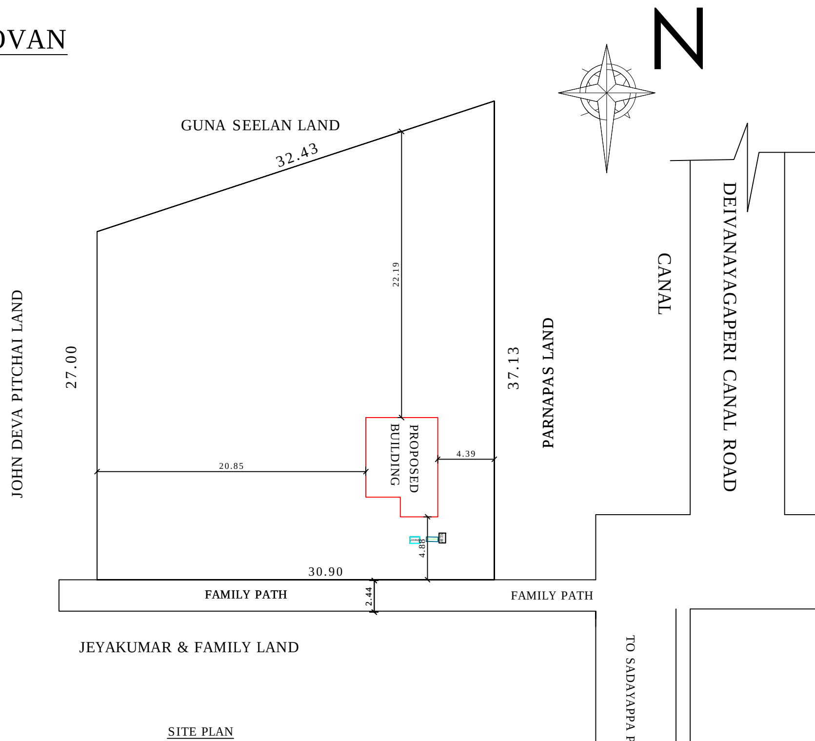
SITE PLAN
