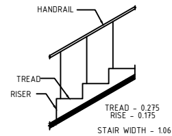
STAIRCASE DETAILS
