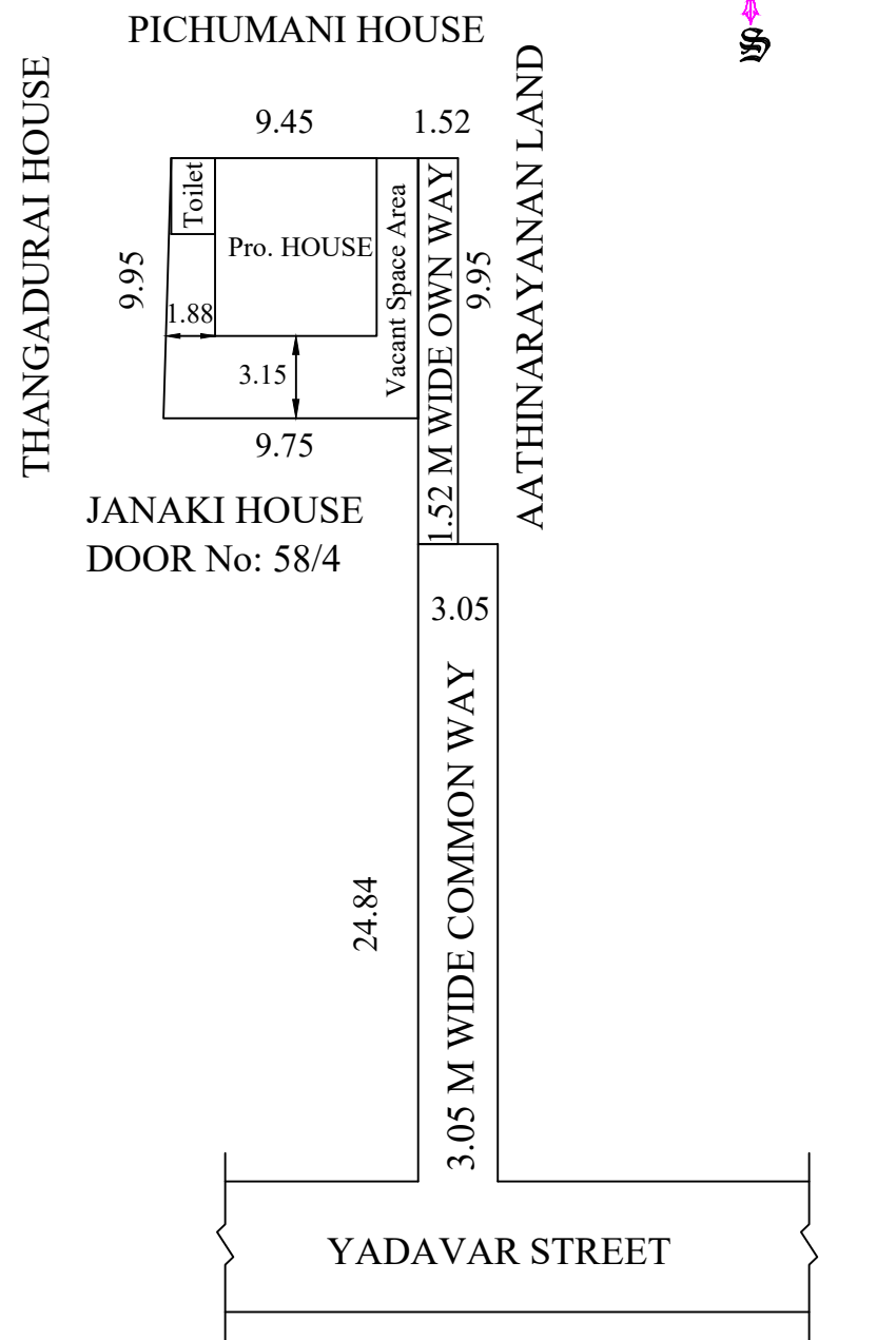
SITE PLAN
