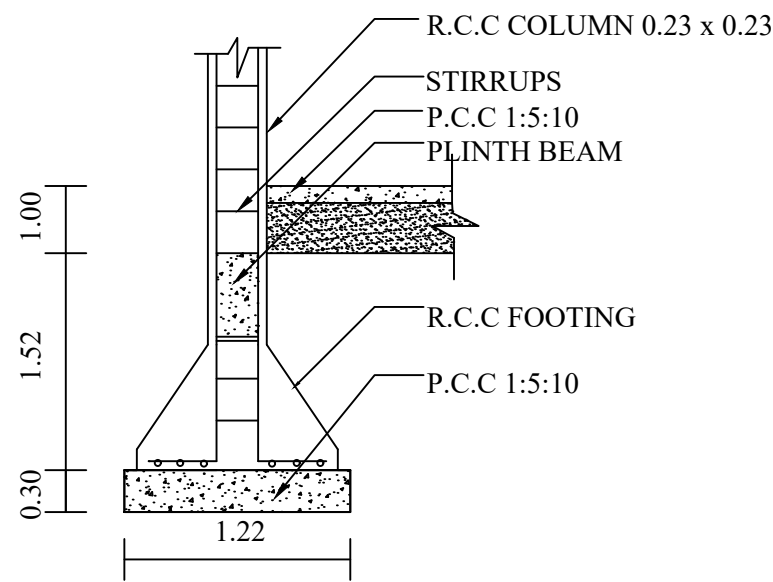
COLUMN DETAILS
