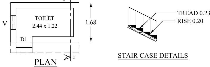
PLAN
