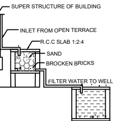
DETAILS OF FILTER BED & WELL
