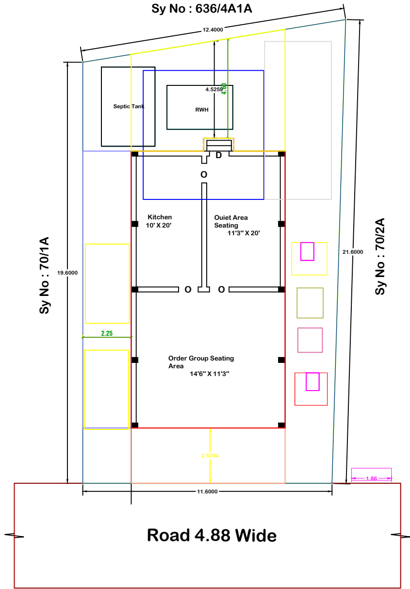
SITE PLAN
