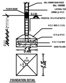
FOUNDATION DETAIL
