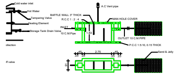
SEPTIC TANK AND TRENCH
