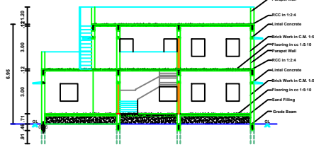
SECTION ON AA'
