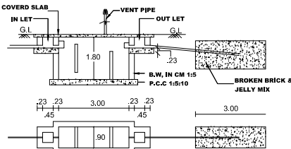
PLAN & SECTION OF SEPTIC TANK & TRENCH
