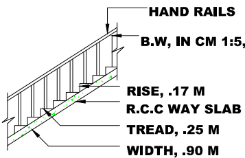
SECTION ON STAIR
