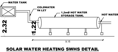
SOLAR WATER HEATING SWHS DETAIL
