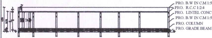
SECTION ON A A
