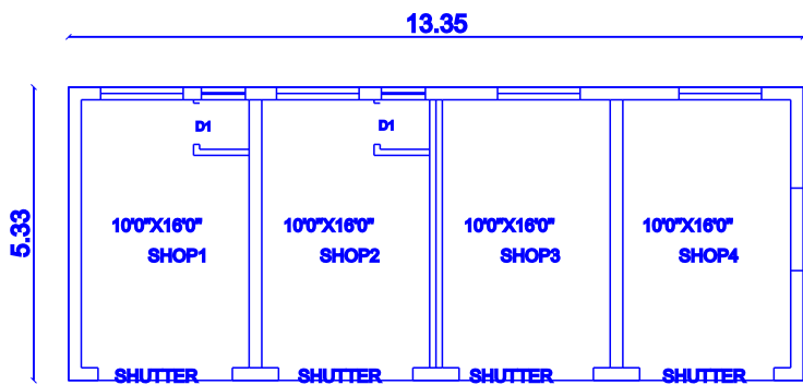
G.FLOOR PLAN
