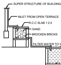
DETAILS OF FILTER BED & WELL
