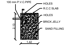
SECTION OF RAIN WATER COLLECTING TANK
