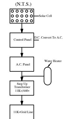
SOLAR SYSTEM
