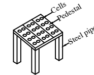
SOLAR SYSTEM
