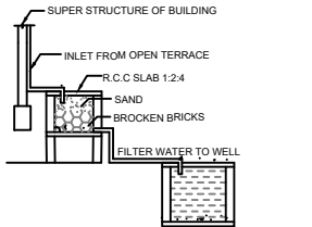
DETAILS OF FILTER BED & WELL
