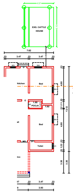
1. & PRO.GROUND FLOOR
