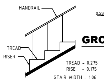
STAIRCASE DETAILS NTS
