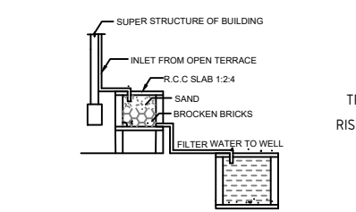
DETAILS OF FILTER BED & WELL NTS
