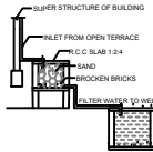
DETAILS OF FILTER BED & WELL
