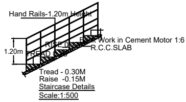
Staircase Details Scale:1:500
