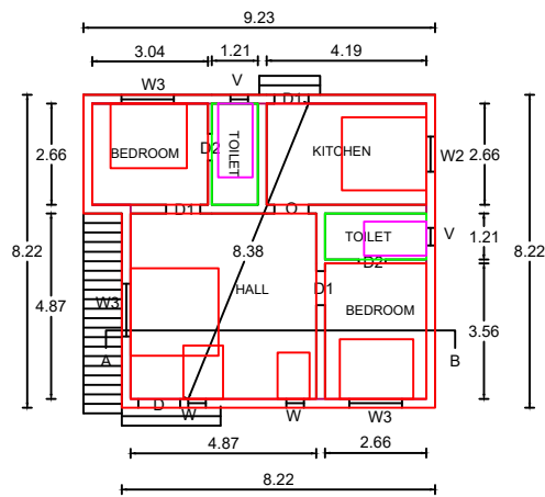
GROND FLOOR PLAN
