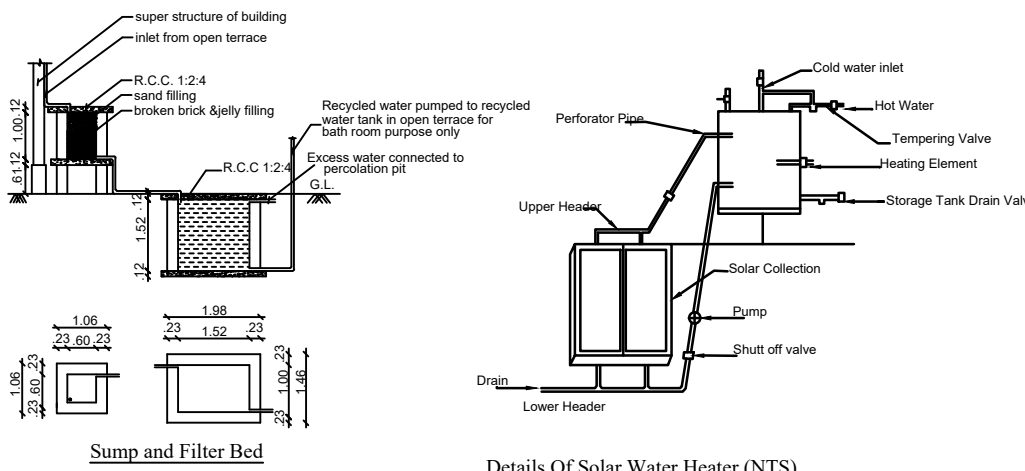
Details Of Solar Water Heater (NTS)
