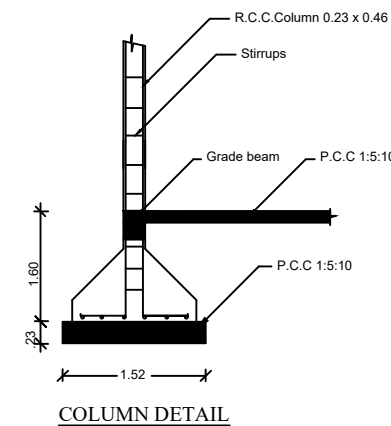
COLUMN DETAIL
