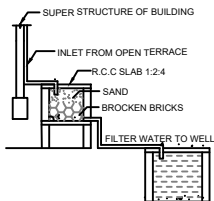
DETAILS OF FILTER BED & WELL NTS
