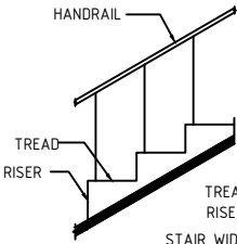
STAIRCASE DETAILS NTS
