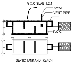
SEPTIC TANK AND TRENCH NTS
