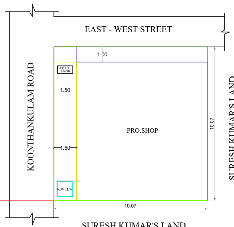
SITE PLAN
