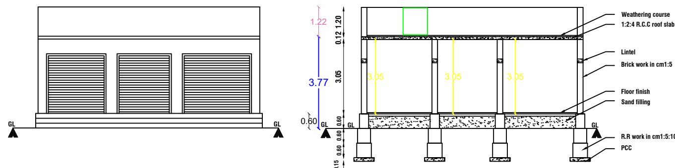
FRONT ELEVATION
