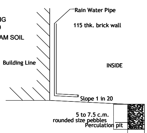
PERCOLATION PIT
