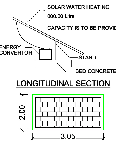
SOLAR SYSTEM
