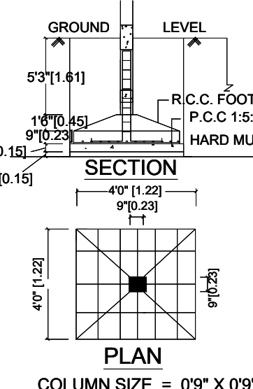
FOUNDATION DETAILS
