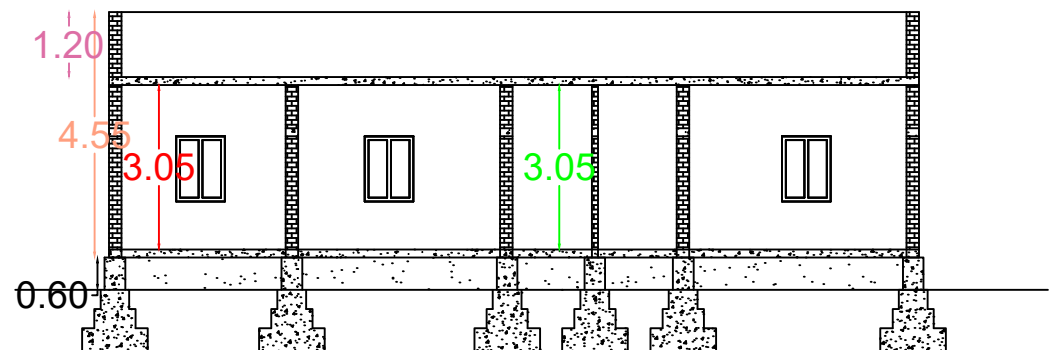
SECTION
