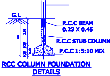
RCC COLUMN FOUNDATION DETAILS
