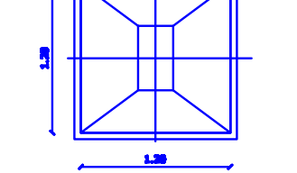
PLAN R.C.C. FOOTING DETAILS
