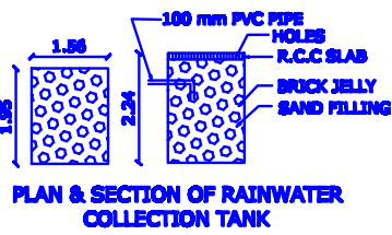
PLAN & SECTION OF RAINWATER COLLECTION TANK
