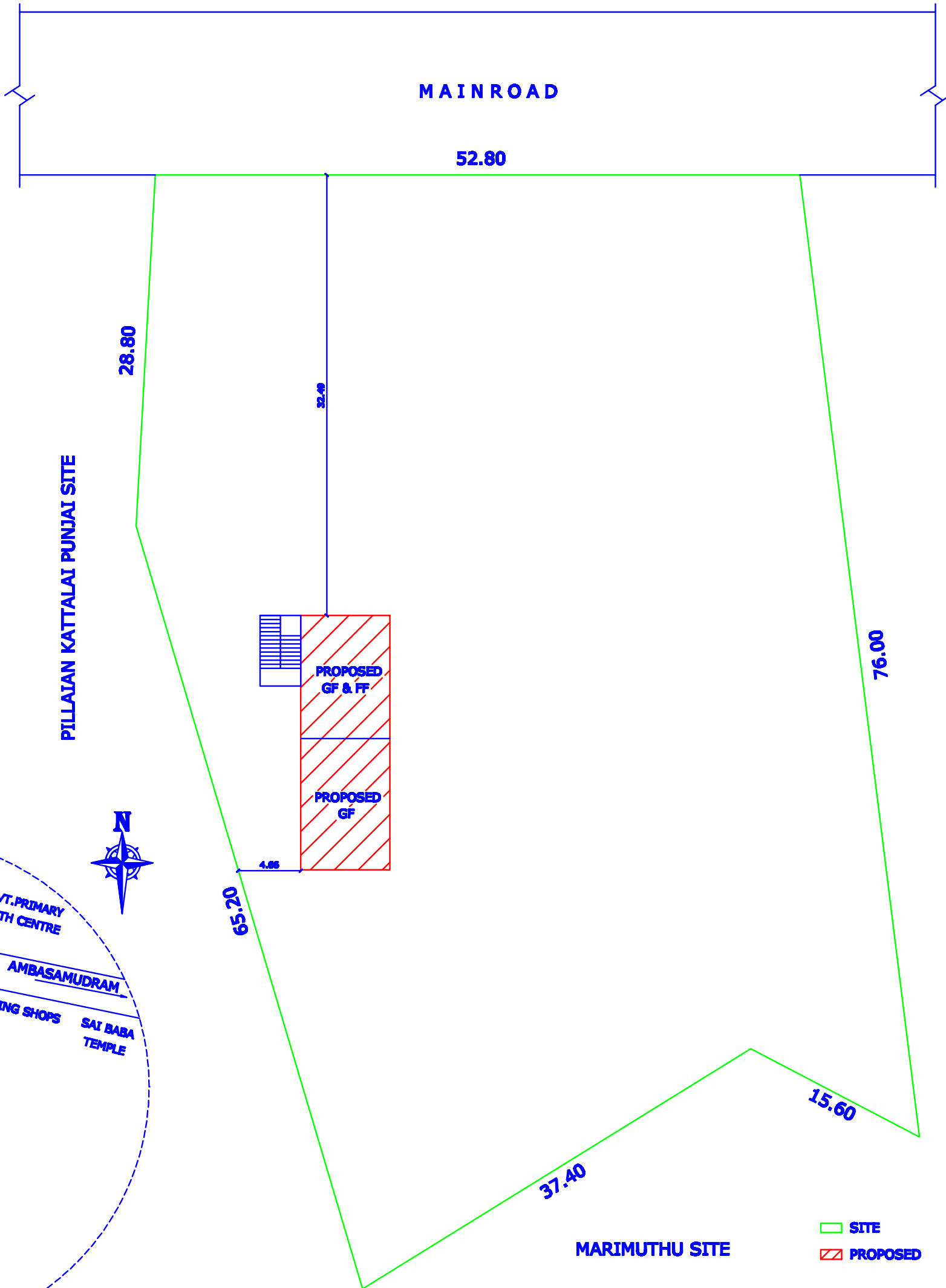
SITE PLAN
