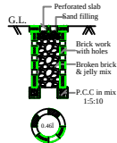
PERCOLATION PIT (NOT FOR SCALE)
