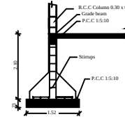
Column Detail
