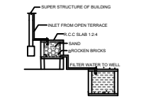
DETAILS OF FILTER BED & WELL
