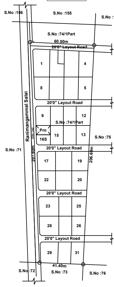
TOPO PLAN (Not To Scale)
