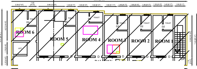
EXISTING APPROVED FIRST FLOOR PLAN
