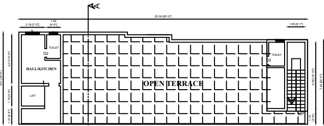
PROPOSED SECOND FLOOR PLAN
